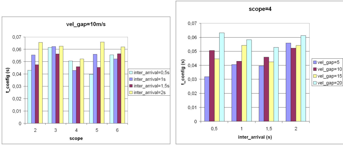
(a) Configuration time per scope for several values of inter_arrival time and with constant vel_gap .
