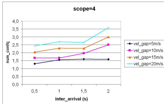
Fig. 11. Number of address configurations of a node per inter_arrival time for several values of vel_gap and with constant scope .
