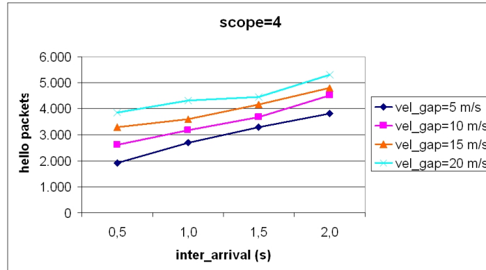
Fig. 10. Number of Hello packets per inter_arrival time for several values of vel_gap and constant scope .
