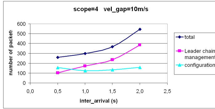
Fig. 12. Number of signalling packets per inter_arrival time for several values of vel_gap and with constant scope .
