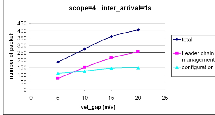
Fig. 13. Number of signalling packets per vel_gap for several values of inter_arrival time and with constant scope .
