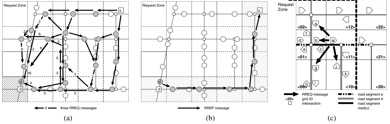
Fig. 2. Route Discovery Process
