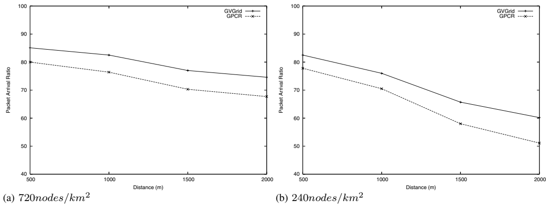
Fig. 8. Average Packet Arrival Ratio
