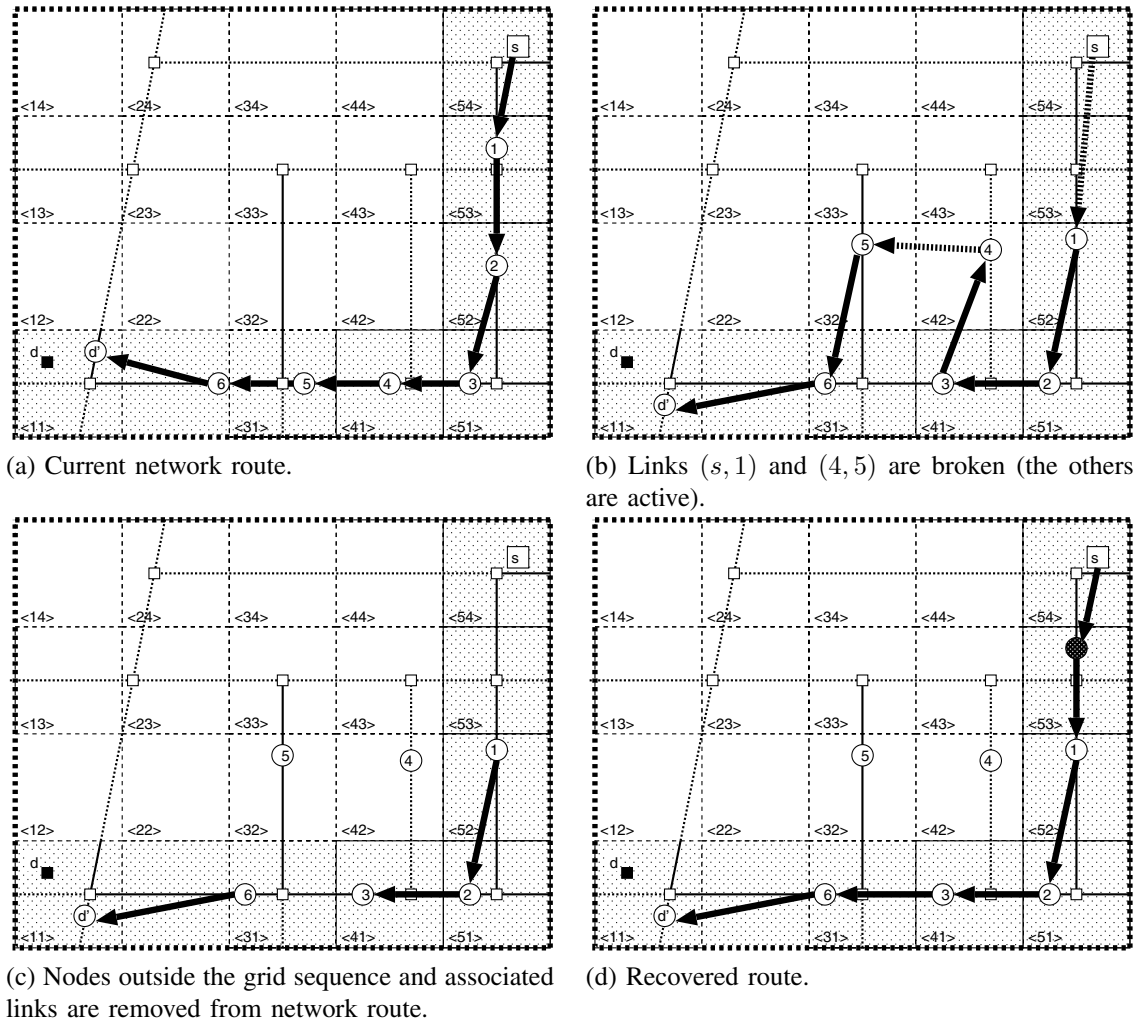
Fig. 6. Route Maintenance Process
