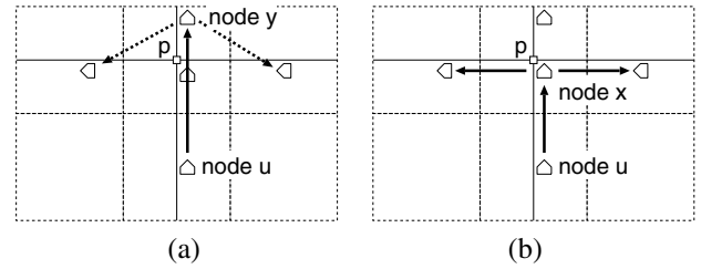
Fig. 3. Effect of Line-of-Sight
