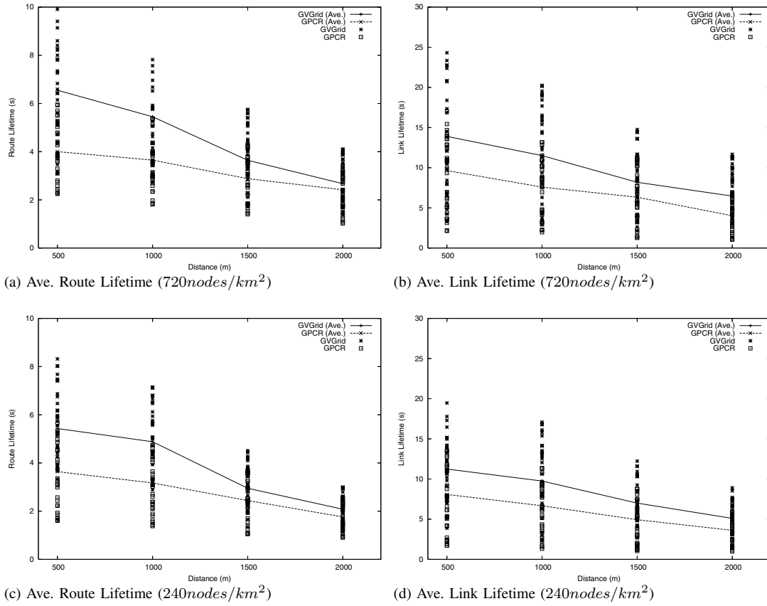
Fig. 7. Route Lifetime and Link Lifetime
