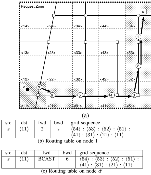
Fig. 5. RREP Message Propagation and Routing Table Update.
