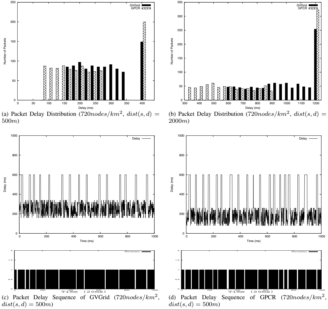
Fig. 9. Packet Delay
