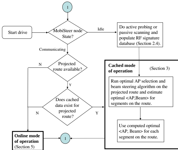
Figure 5: MobiSteer operation.
