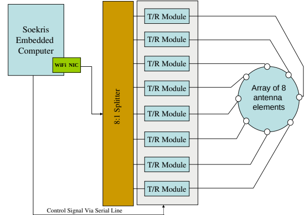
Figure 2: Block diagram of directional antenna components.
