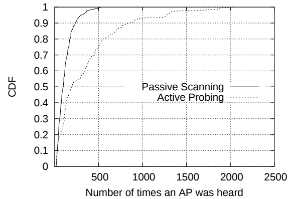
Figure 6: Performance of active probing vs. passive scanning in building RF signature database.
