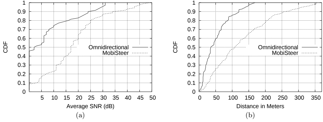
Figure 13: (a) Average SNR from In Situ APs in each 40 meter segment along the route with beam steering and with omni-directional beam. (b) Distance along the route each AP was heard with beam steering and with omni-directional beam.
