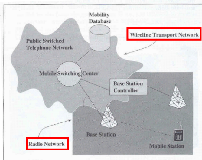
Figure 1.1 The basic PCS network architecture.
