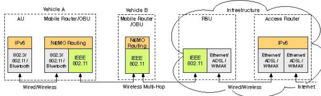
Fig. 4. Protocol stack for NEMO-centric approach
