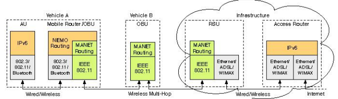
Fig. 3. Protocol stack for MANET-centric approach
