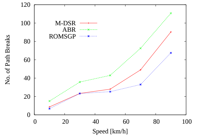
Fig. 9. Number of path breaks when varying the speed of vehicles (communication range = 400 m).
