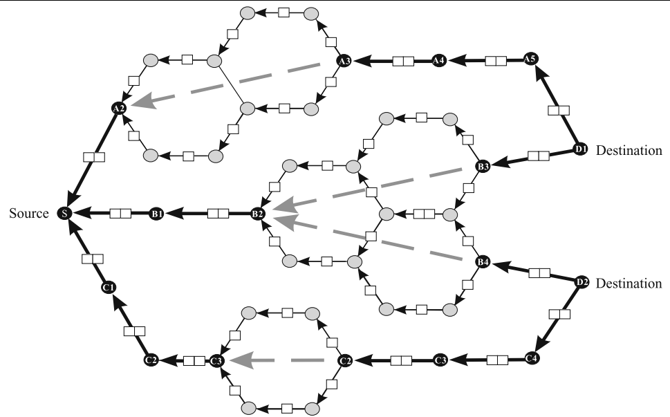
Fig. 13 Hexagonal-tree reply
