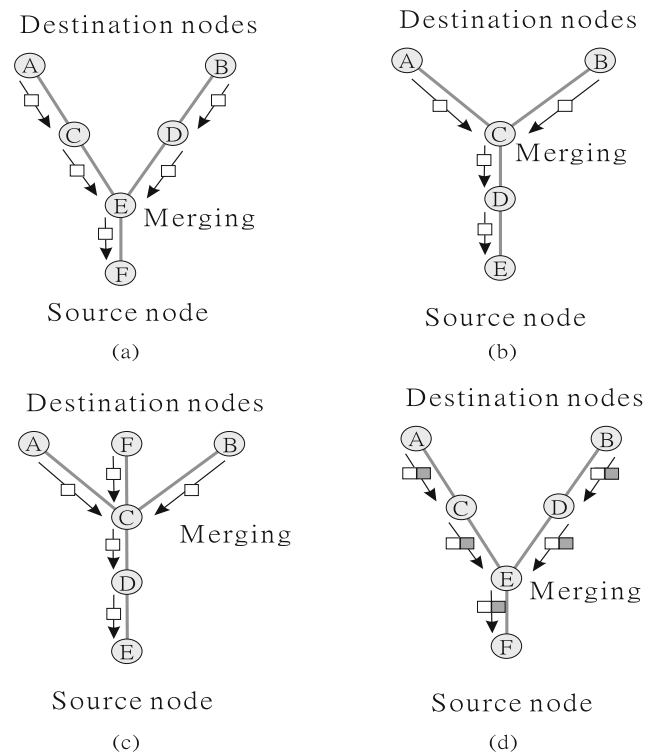
Fig. 14 Merging examples
