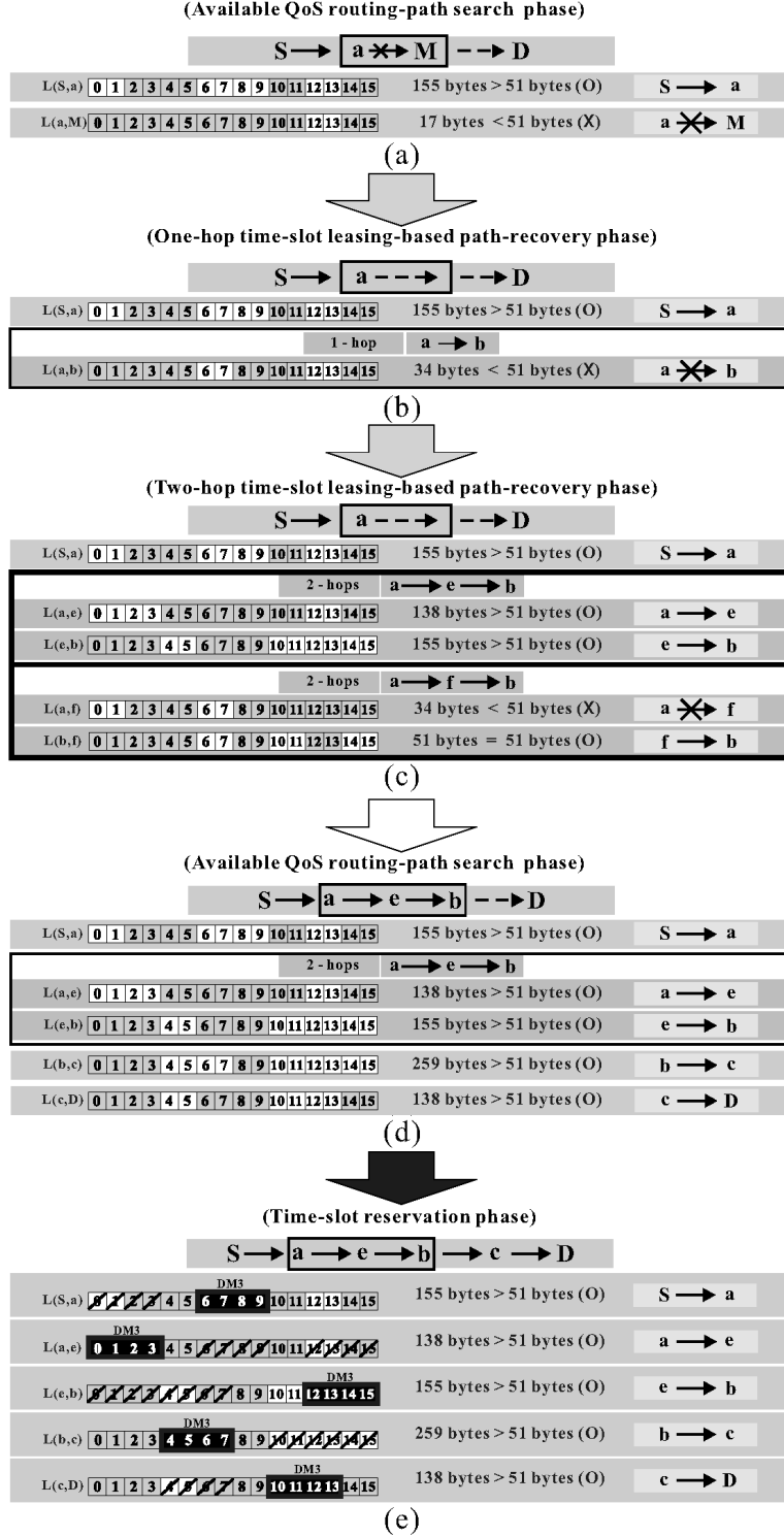
Figure 9 Time-slot reservation steps using the twohop CTQ approach
