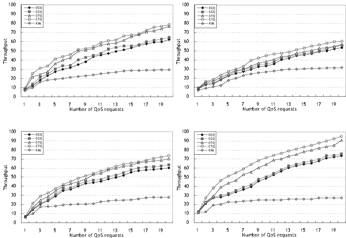
Figure 16 Throughput vs. the number of QoS requests (a) DM1:DM3:DM5 = 1:1:1 , (b) DM1:DM3:DM5 = 3:1:1 , (c) DM1:DM3:DM5 = 1:3:1 and (d) DM1:DM3:DM5 = 1:1:3
