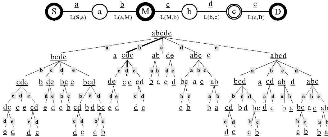
Figure 11 Conditions of time-slot reservation with a normal optimal algorithm
